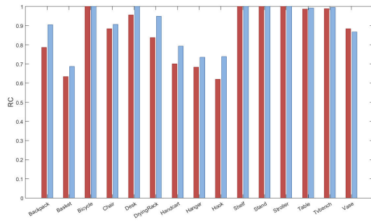
Figure 12: Results of a user study where the bars show the agreement of our functionality score with the score derived from users. The agreement is computed for each category in terms of the RC.
