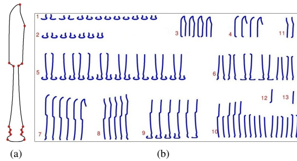
Figure 3: Per-shape curve feature extraction. (a) 16 curvature extrema (red dots) are detected along the contour of a knife, which are later used to extract 93 curve segments. (b) 13 per-shape feature modes are generated by clustering all these curve segments.
