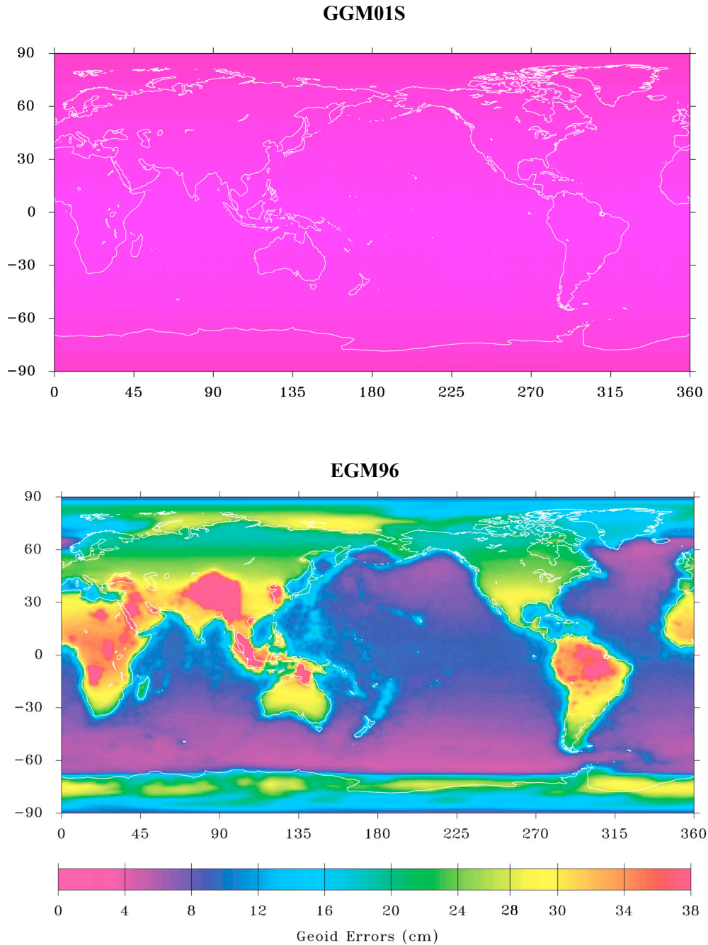
Figure 2: Geoid error predicted by the full covariance as a function of geographic location for GGM01S and EGM96 to degree and order 70 shown on the same scale. Due to the global, homogeneous nature of the GRACE data, the resulting geoid errors show no discrimination between land or sea (upper panel) as do previous gravity models (lower panel). The GGM01S geoid is estimated to be accurate to approximately 2 cm to degree and order 70 (300 km resolution) and 6 cm to degree and order 90 (200 km resolution).
