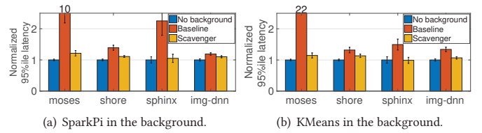
Figure 9: Performance degradation of individual TailBench workloads in Lab testbed collocated with Spark.
