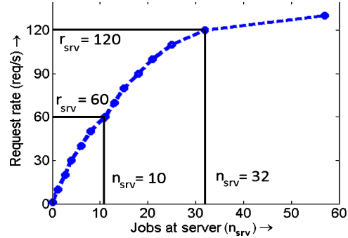
Fig. 14. A doubling of request rate can lead to a tripling of number of requests at a single server.
