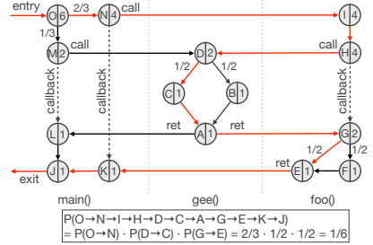
Fig. 6. Weighted iCFG for Fig.5
