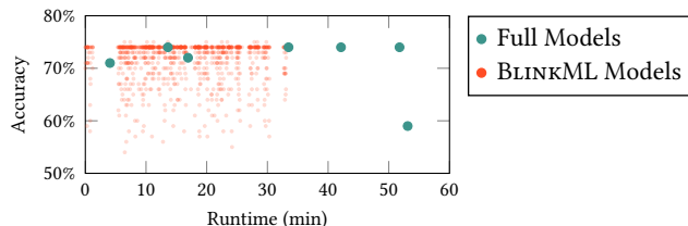
Figure 10: Hyperparameter optimization
