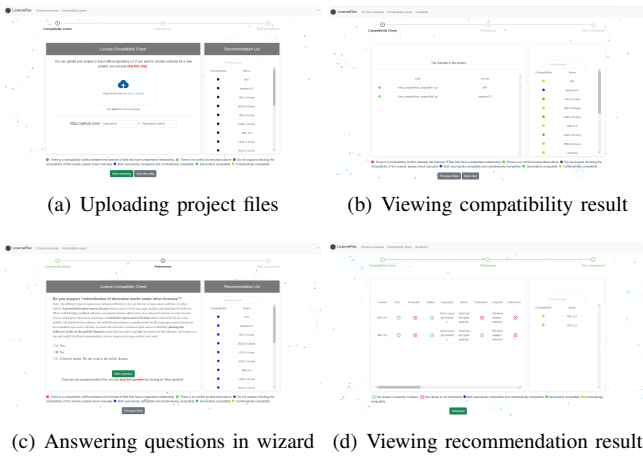
Fig. 1. LicenseRec interfaces for developers to choose a license.
