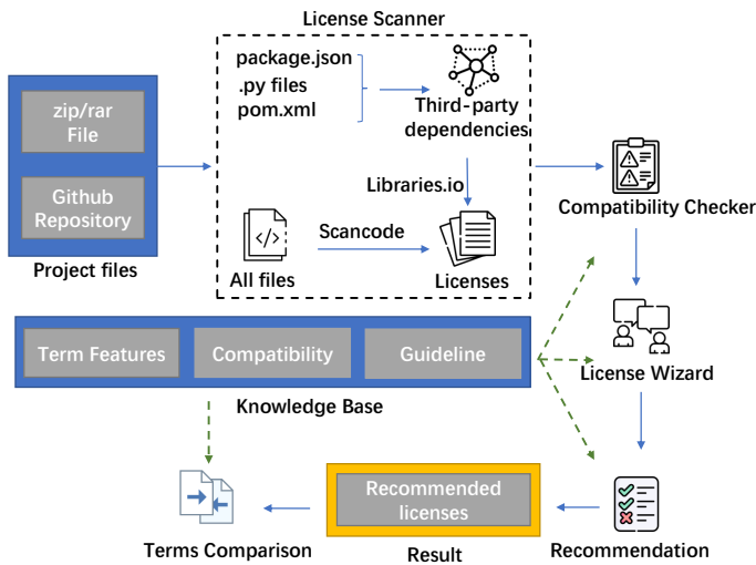
Fig. 2. Overview of LicenseRec.
