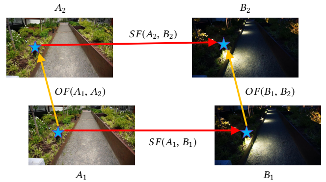
Fig. 5. Illustration of loop consistency check.
