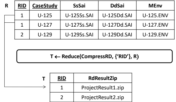
Figure 5. An example of Reduce.
