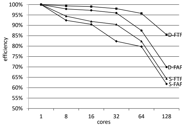
Figure 10. Evaluation of RFA workflow with 700 case studies.
