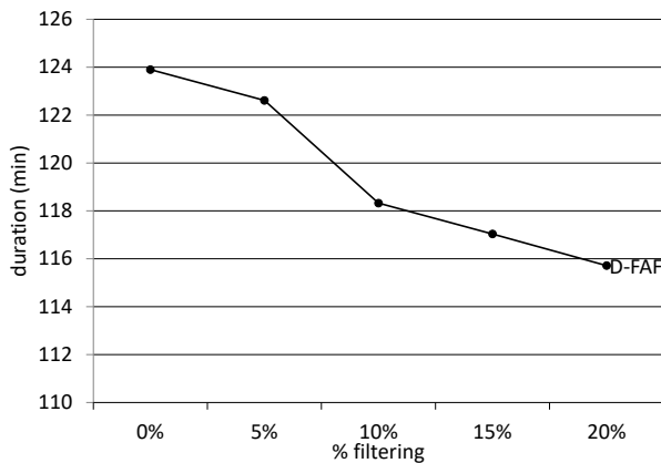
Figure 11. Optimization of RFA workflow.
