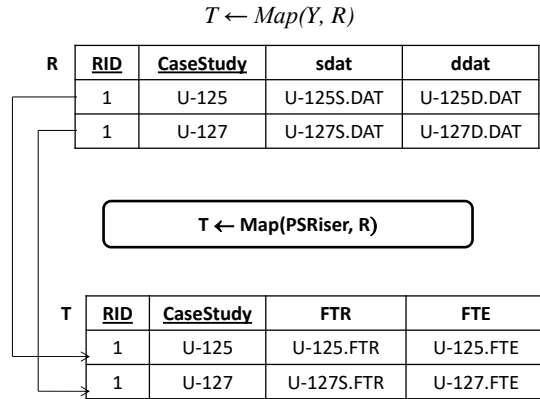
Figure 4. An example of Map.
