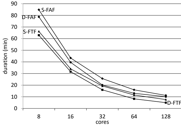
Figure 9. Evaluation of RFA workflow with 358 case studies.
