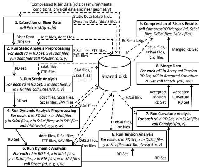
Figure 1. Risers Fatigue Analysis (RFA) scientific workflow.
