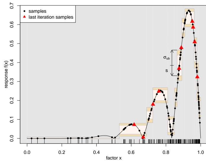
Figure 3.7: HVS on a synthetic 1D benchmark after fifteen drawings of ten samples each. The true response, f(x) = x^5|\sin(6\pi x)| , is the solid line. CART partitions the factor dimension into intervals, represented by the boxes horizontal extension. For each interval, the estimated standard deviation, s , is in a light color and the upper bound of the standard deviation, \sigma_{ub} , is dark. HVS selects more samples in the irregular regions.
