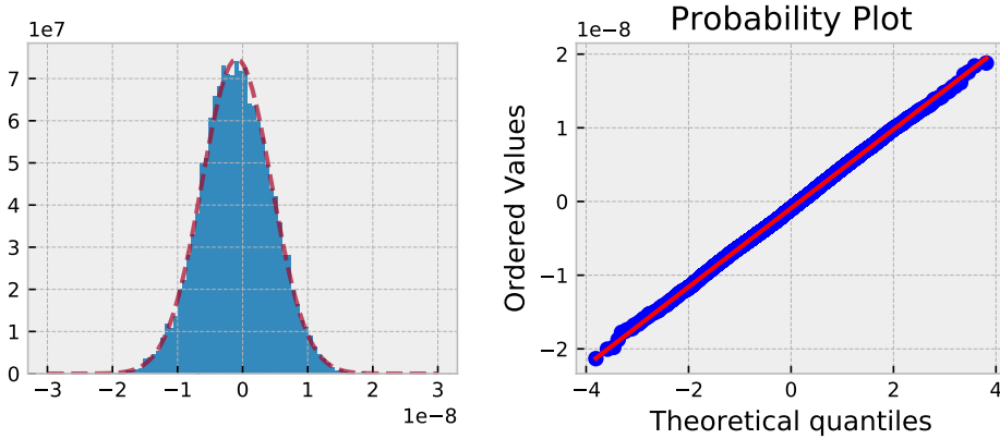
Figure 5.2: Normality of Cramer X[0] sample
