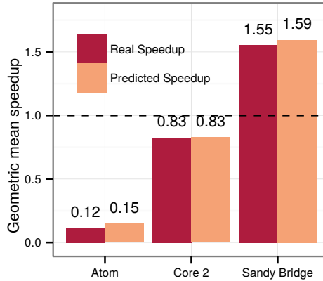
Figure 3.5: NAS geometric mean speedup on three architectures. Baseline is a NAS run on Nehalem compiled with icc 12.1.0 -O3 -xsse4.2 . The predicted speedup is computed by using the replay performance of eighteen CERE representative codelets using Working Set warmup.
