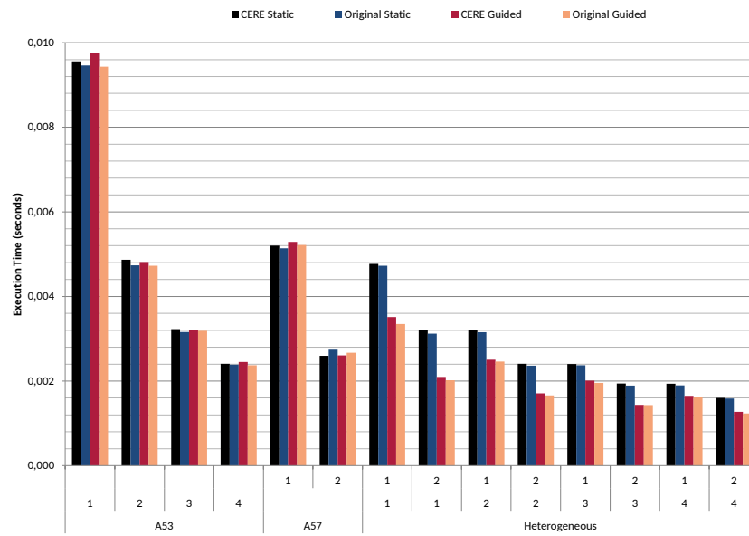
Figure 4.5: Execution time of PARSEC Blackscholes 64K in a Juno board. The horizontal axis shows the thread mapping across the four A53 and two A57 cores. The numbers in the first (respectively second) line are the number of threads mapped on A57 (respectively A53) cores. The first two categories consider homogeneous mappings, and the last category considers heterogeneous mappings. For each mapping, we both consider static and guided scheduling strategies. For each scheduling, we validate the time estimated by CERE to the time measured in the original benchmark.
