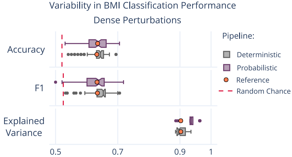
Figure 7.7: Variability in BMI classification on an MCA RR perturbed connectome.
