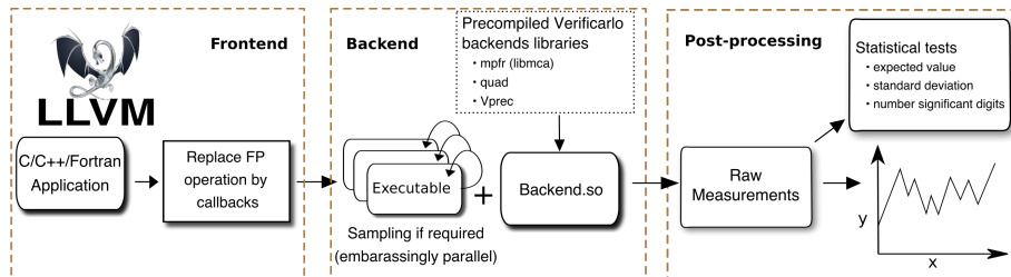
Figure 6.1: Bird’s eye view of the verificarlo pipeline.
