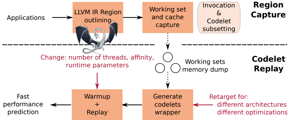
Figure 2.1: CERE workflow. Applications are partitioned into a set of codelets, which may be pruned using different criteria. A set of representative invocations are selected and captured. The codelets can then be replayed with different options and on different targets.
