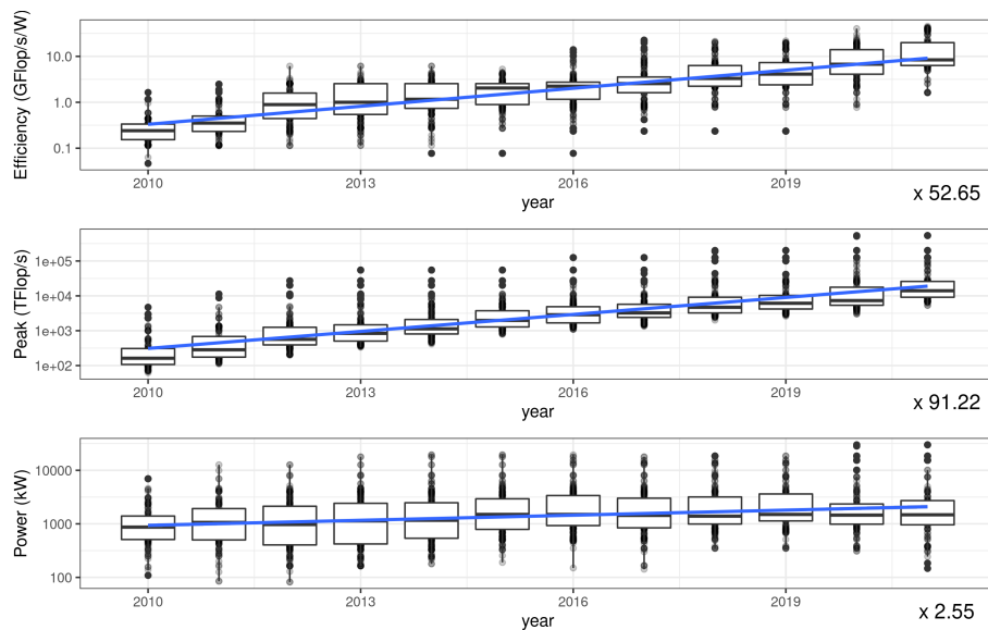
Figure 8.1: Evolution over time of the first 100 systems in the TOP500 list. Peak is the theoretical peak computing performance. Each point is an HPC system. Box plots span from the first to the third quartile. The blue line is a linear regression on the individual HPC systems' metrics. Because the vertical axis is logarithmic, Peak and Efficiency follow roughly a geometric growth.
