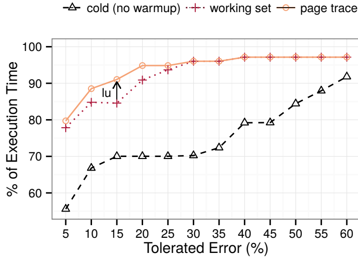
Figure 2.9: Comparison of the three cache warm up techniques included in CERE on NAS codelets. The plot shows the percentage of execution time as a function of the replay error. Page Trace and Working Set warm up achieve the best results. Page Trace is more accurate than Working Set on the LU benchmark.
