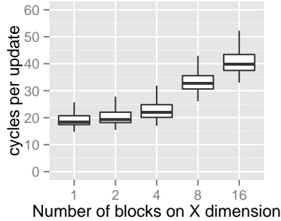
Figure 4.10: Performance of different X blocking configurations. The size of the blocks is inversely proportional to the number of blocks. Large block sizes across X exhibit the best performance.
