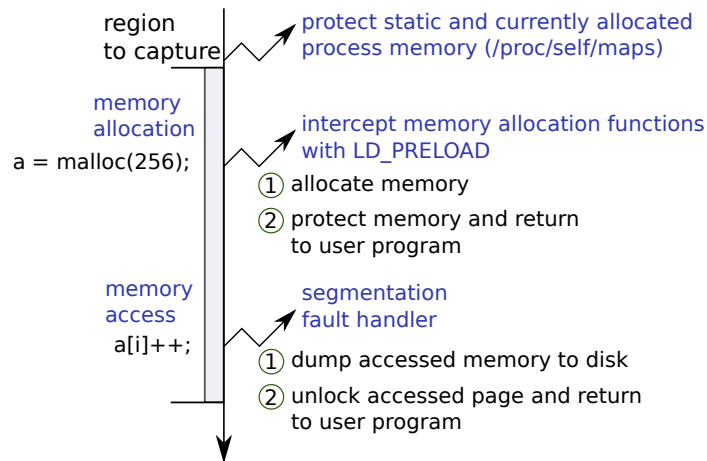
Figure 2.5: The memory dump process operates at page granularity. Each page accessed is dumped by intercepting the first touch using memory protection support.
