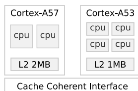
Figure 4.4: Juno big.LITTLE ARM architecture
