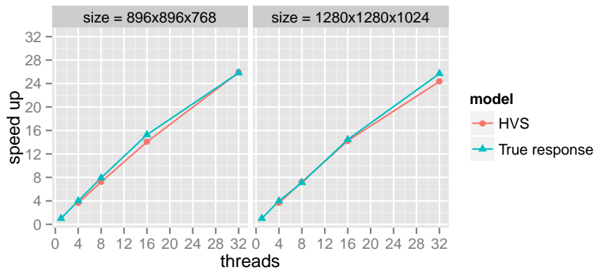
Figure 4.12: Scalability for the isotropic-split implementation with half order p = 4 , NX = 1 , NY = 128 , and NZ = 32 . The speedup is computed using the single thread performance with the same parameters.
