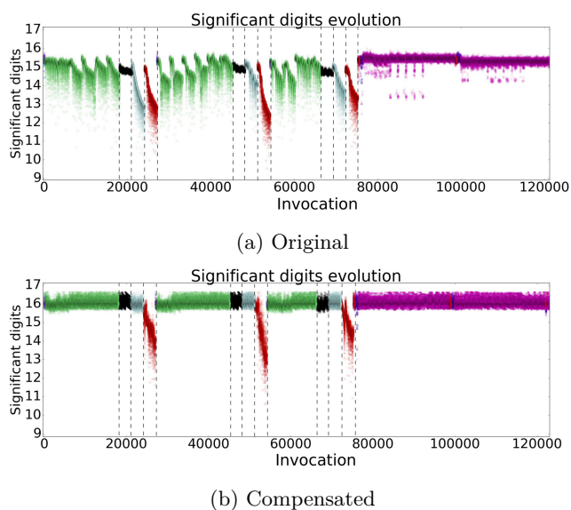
Figure 6.7: Profiles produced by VeriTracer of simp_gen . Several accuracy losses present in the original version (a) are improved by the compensated algorithm Dot2 (b). Each color maps one of the 31 distinct call-site paths. Dot2 improved 30 out of 31 call-site paths.
