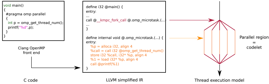
Figure 2.4: Clang outlines each C parallel region as an independent IR function: omp_microtask . The call to kmpc_fork spawns a pool of threads that runs the outlined microtask.
