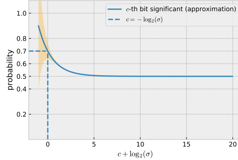
Figure 5.7: Profile of the contribution bit curve: when the dashed line is positioned on the -\log_2 \sigma abscissa, the curve corresponds to the approximation 5.12 of the probability that the bit contributes to the result accuracy. The shaded area represents the bound on the error given by equation 5.13.
