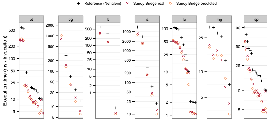
Figure 3.3: Predicted and Real execution times on Sandy Bridge compared to the Nehalem reference execution. Each box presents the codelets extracted from one of the NAS applications. Only three codelets in BT, LU, and SP are mispredicted.
