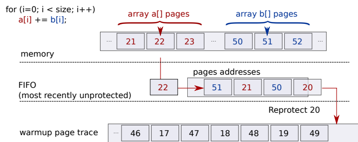
Figure 2.8: Cache page tracer on a simple codelet adding two arrays. Each page access is logged. Recently unprotected pages are kept in a FIFO with N slots (here N = 4 ). Once evicted from the FIFO, the pages are protected again.
