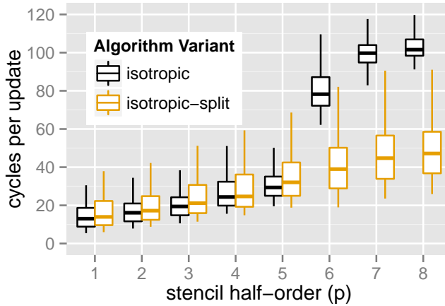
Figure 4.9: Performance of the isotropic and isotropic-split code variants. For p larger than five, the isotropic-split version is significantly faster.
