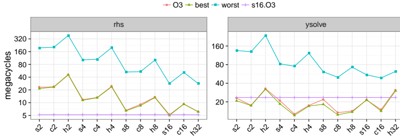
Figure 4.1: Tuning exploration for two SP regions. For each affinity, we plot the best, worst, and -O3 optimization sequences. Custom optimization beats -O3 for s2,s4 , and s8 on ysolve .
