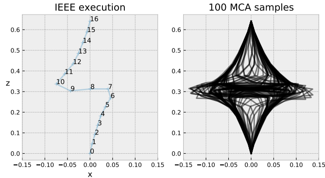
Figure 7.1: Europlexus buckling simulation of a doubly clamped column subject to a vertical pressure. The nodes of the column are labeled in the plot from 0 to 16. The left plot shows the deterministic and reproducible results produced by an IEEE-754 run of the simulation. In the right plot, a two-digits numerical error is simulated by collecting one hundred MCA samples with verificarlo ( t = 50 ). The buckling direction is completely dominated by the small numerical error introduced.
