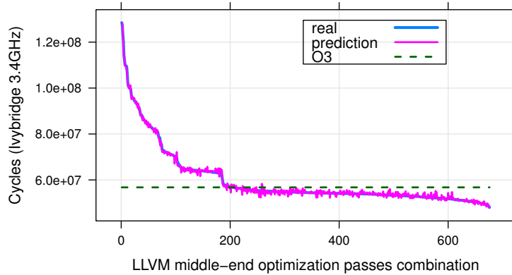
Figure 4.2: NAS SP ysolve region execution time across 1000 schedules of random compiler combinations passes based on O3. Compilation sequences are sorted according to their original execution time. We remove compilation sequences that produce the same binary. real and predicted respectively represents the original execution time and the codelet prediction based on representative invocations replay. The codelet faithfully predicts the region execution time across the different compiler optimizations.
