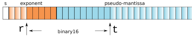
Figure 6.6: By setting e = 5 and t = 10 , VPREC simulates a binary16 embedded inside a binary32 . Opaque bits represent the new exponent range and precision available. The sign remains the same.
