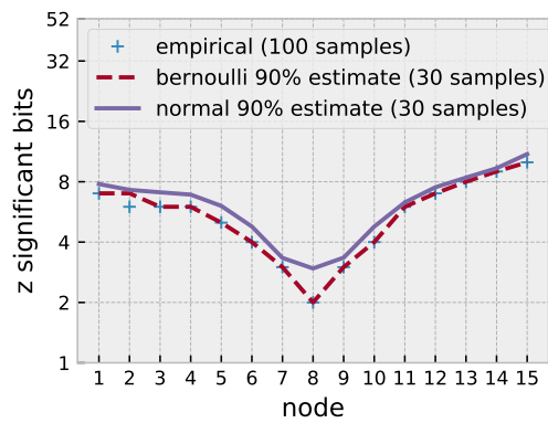
Figure 7.3: Significant bits on the z axis distribution. Bernoulli's estimation precisely captures the behavior (except for node 2). The normal formula overestimates the number of digits; this is expected since the distribution is strongly non-normal.
