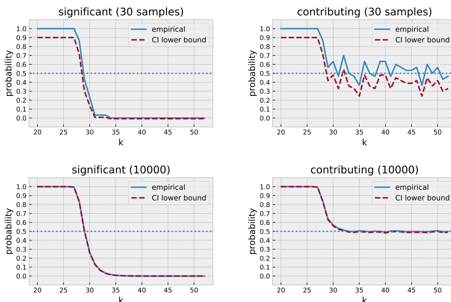
Figure 5.10: Significance and contribution per bit for variable X[0] of the Cramer's system with 30 and 10000 samples.
