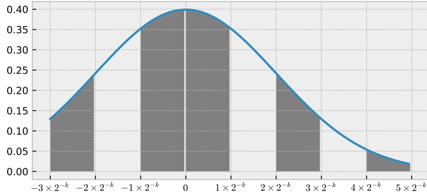
Figure 5.6: Normal curve; the gray zones correspond to the area where the k -th bit contributes to make the result closer to 0 (whatever the preceding digits).
