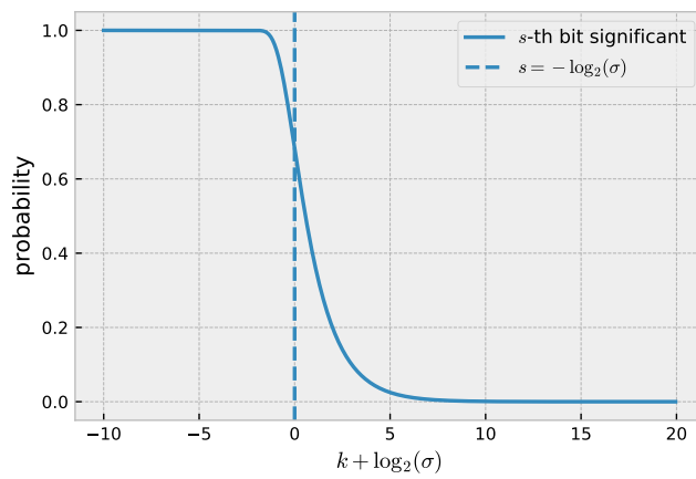
Figure 5.4: Profile of the significant bit curve: when the dashed line is positioned on the -\log_2 \sigma abscissa, the curve corresponds to the probability that the result is significant up to a given bit.
