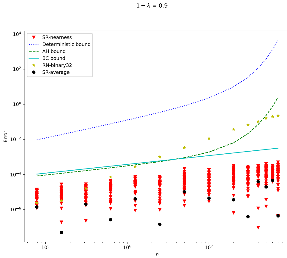
Figure 7.11: Probabilistic bounds with probability 1 - \lambda = 0.9 vs deterministic bound of the computed forward errors of the inner product with u = 2^{-23} .
