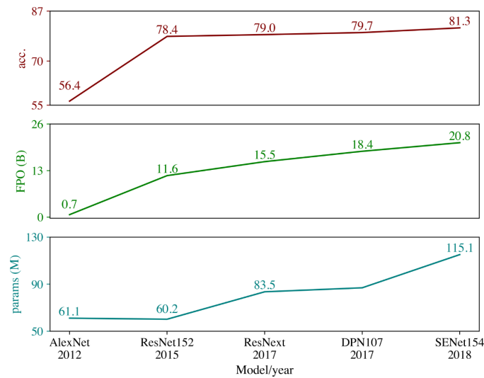
Figure 8.3: Accuracy (acc.) vs. computation (FPO) for AI neural networks identifying objects in the ImageNet dataset. Figure from Schwartz et al. [178]. acc. is the top-1 accuracy percentage. FPO is the total number of floating point operations required for training the network. params is the number of model parameters.
