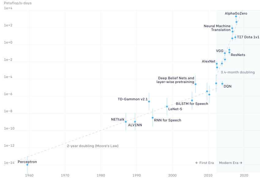
Figure 8.2: Computation power required to train AI systems, data and figure by OpenAI [25]. From 2012, AI computation demands have become steeper doubling every 3.4 months.
