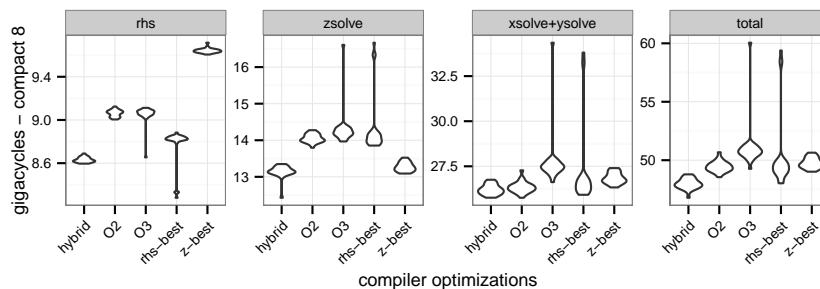
Figure 4.3: Violin plot execution time of SP regions using best NUMA affinity. Measures were performed 31 times to ensure reproducibility. When measuring total execution time, hybrid compilation outperforms all other optimization levels, since each region uses the best available optimization sequence.
