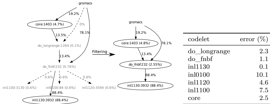
Figure 2.2: ( left ) CERE call graph, before and after filtering, for SPEC 2006 gromacs. Each node represents a captured codelet. The percentage inside the node is the codelet’s self time. Edges represent calls to other codelets, the edge percentage is the time spent in calls to those nested codelets. ( right ) Replay percentage error of gromacs codelets using Working Set warmup.
