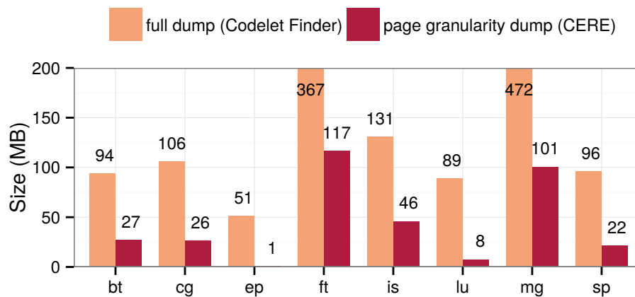
Figure 2.6: Comparison between the page capture and full dump size on NAS.A benchmarks. CERE page granularity dump only contains the pages accessed by a codelet. Therefore, it is much smaller than a full memory dump.
