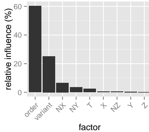
Figure 4.8: Relative influence of input factors in the FDTD kernel. The influence determines how much a factor affects the response. For the GBM model, it is computed as described in [79].
