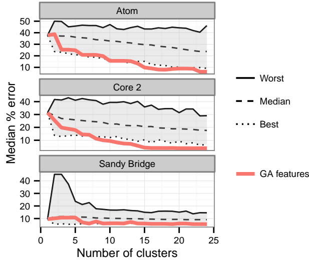
Figure 3.4: Genetic-Algorithm feature clustering compared to random clustering. For each number of clusters, from 2 to 24, 1000 random clusters are evaluated. Clustering with our GA feature set is consistently close or better than the best random clustering (out of 1000).
