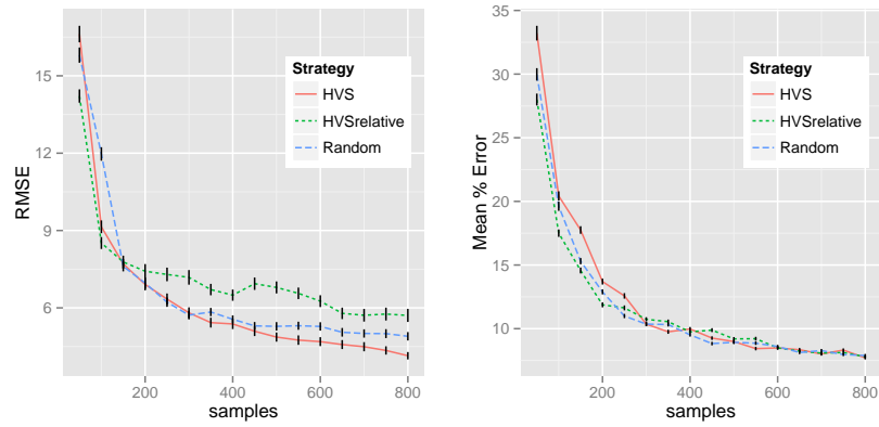
Figure 4.7: Root mean square error and Mean percentage error for the three tested strategies in the FDTD case study. The error is evaluated against a randomly selected test set of 3225 points. The vertical black lines show the bootstrap confidence intervals.
