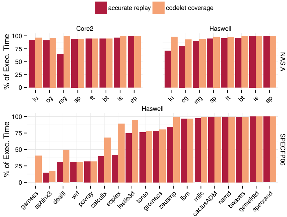
Figure 2.11: Evaluation of CERE on NAS and SPEC FP 2006. The Coverage is the percentage of the execution time captured by codelets. The Accurate Replay is the percentage of execution time replayed with an error less than 15%.
