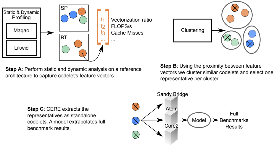
Figure 3.2: Overview of the benchmark reduction method for execution time prediction. The reduction method can be extended to support compiler or optimization evaluation.
