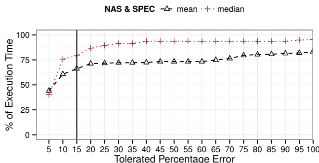
Figure 2.3: Mean and median captured execution time as a function of the tolerated replay error on the NAS and SPEC 2006 FP benchmarks. The mean is lower than the median due to the IO-intensive and short kernel benchmarks described in section 2.4, which skew the distribution.
