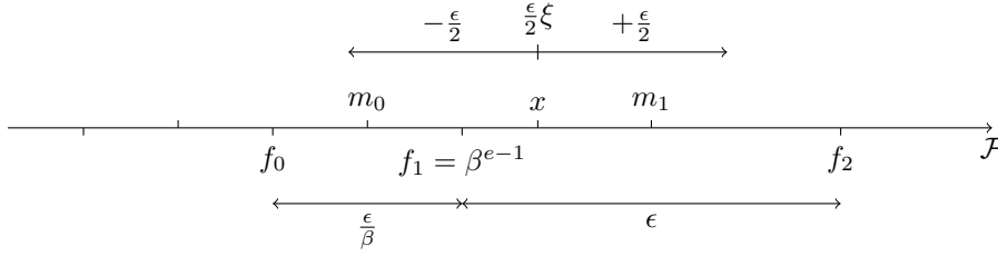
Figure 5.3: Rounding carry-out when x is close to a power of the base.
