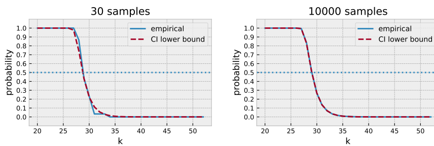
Figure 5.5: Significant bits for Cramer x[0] variable computed under the normal hypothesis using 30 and 10000 samples. The Confidence Interval (CI) lower bound is computed by using the probability of theorem 5.5.1 and bounding \sigma with a 95% Chi-2 confidence interval.
