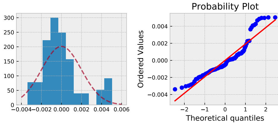
Figure 7.2: Non normality of buckling samples on z axis and node 1. Shapiro Wilk rejects the normality hypothesis.
