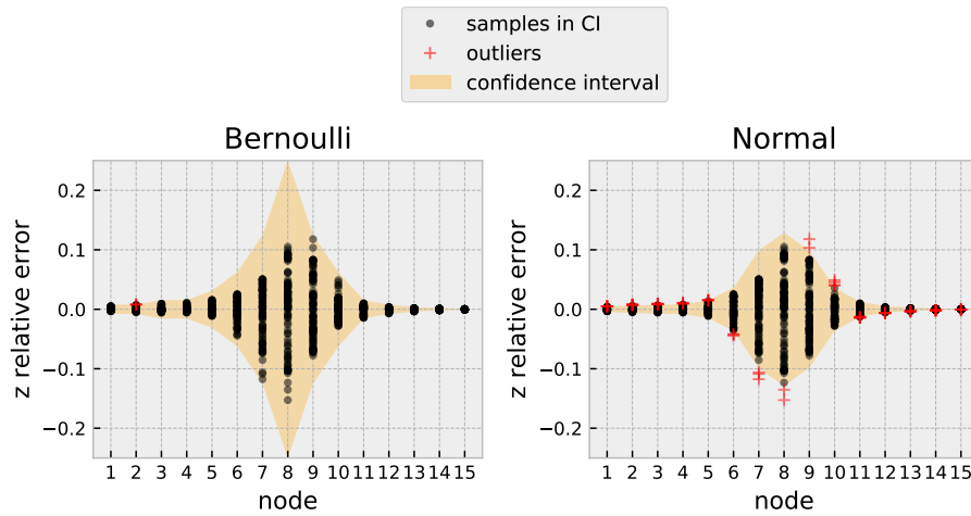
Figure 7.4: Relative error between the samples and the mean of the z -axis distribution. The shaded envelope corresponds to the computed confidence interval with 30 samples. Black dots are samples that fall inside the CI. Red crosses are outliers that fall outside the CI. In the Bernoulli case, only 3 samples out of 70 fall outside of the interval; which is compatible with the 90% probability threshold.
