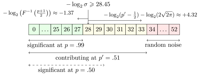
Figure 5.9: Summary of results on the X[0] Cramer example. 28.45 \approx -\log_2 \hat{\sigma} - \frac{1}{2} \log_2 \left( \frac{n-1}{\chi_{1-\alpha/2}^2} \right)
