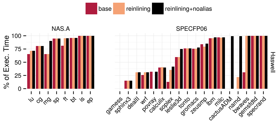
Figure 2.12: Percentage of execution time accurately replayed (error < 15%) on the NAS and SPEC FP benchmarks with different replay configurations. Reinlining and explicitly marking cloned variables as NoAlias improve replay accuracy in eleven benchmarks.
