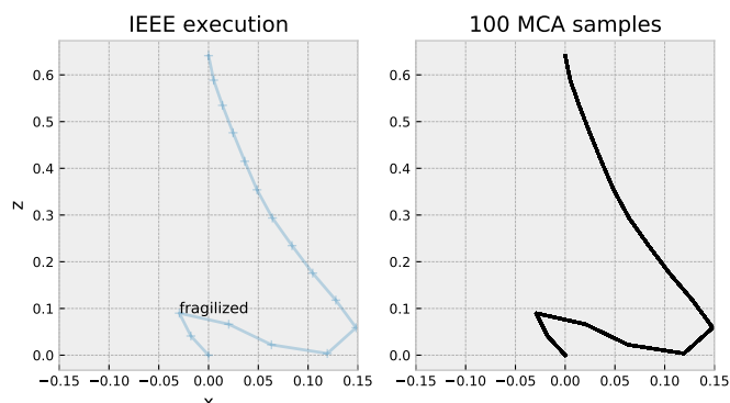
Figure 7.5: Europlexus buckling simulation with a fragilized node 2. By weakening the column, the physical process becomes reproducible in the presence of small numerical noise.
