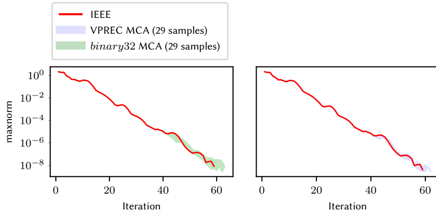
Figure 7.9: Resiliency of VPREC and binary32 configurations. In red is the IEEE maxnorm convergence for reference. The blue envelope shows the 29 MCA samples for the previously found VPREC configuration. Green envelop shows the 29 MCA samples for the binary32 configuration. All samples converge, showing the resiliency of both configurations.
