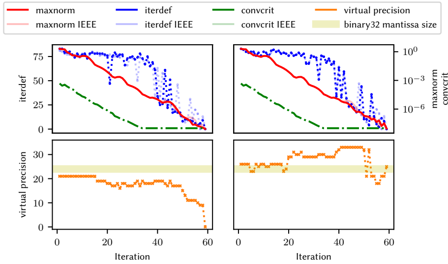
Figure 7.8: Adaptive precision searching on YALES2’s DPCG with the deflated part ( left ) and the entire code ( right ). On both plots, we can see that our reduced precision solution follows the reference IEEE convergence profile.
