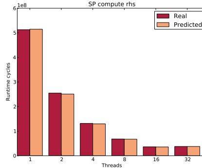
Figure 2.13: Real vs. PCERE execution time predictions on Sandy Bridge for the SP compute rhs codelet
