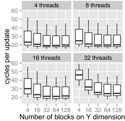
Figure 4.11: Performance of different Y blocking configurations. For a high number of threads, reducing the Y block size improves performance.
