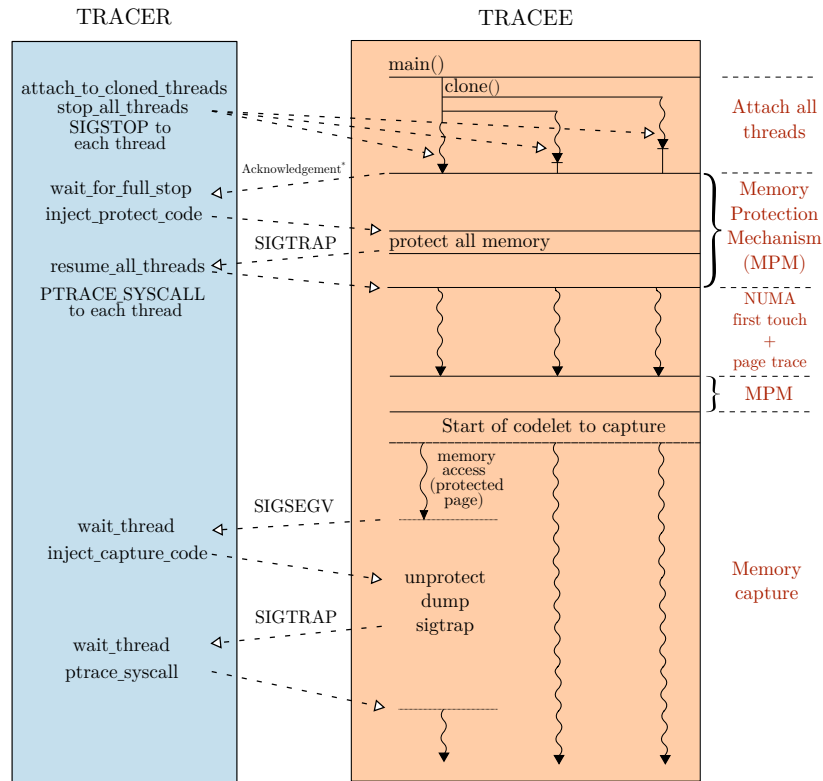
Figure 2.7: Multithreaded capture mechanism with ptrace. Capture is split into two distinct processes: the CERE capturing method as the tracer the studied application as the tracee.
