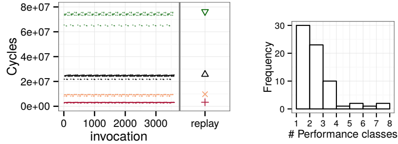
(a) SPEC tonto make_ft@shell12.F90:1133 execution trace.
