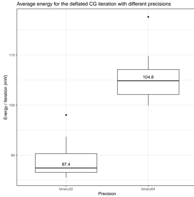
Figure 7.10: Energy per iteration of the deflated CG for a single Yales2 process (measured on an Intel Core i7-4770).
