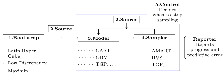
Figure 3.6: ASK pipeline
