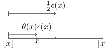
Figure 5.1: \theta(x) is the fraction of \epsilon(x) to be rounded away.
