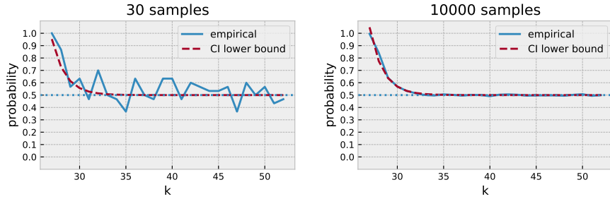
Figure 5.8: Contributing bits for Cramer x[0] variable computed under the normal hypothesis using 30 and 10000 samples with the approximation of equation 5.12.
