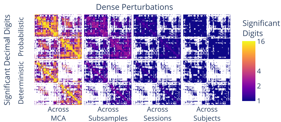
Figure 7.6: Significant digits in connectomes across MCA samples, subsamples, sessions, and subjects.
